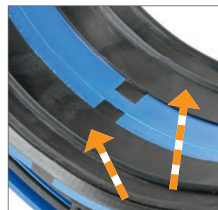
double security with the 2-profile sealing
